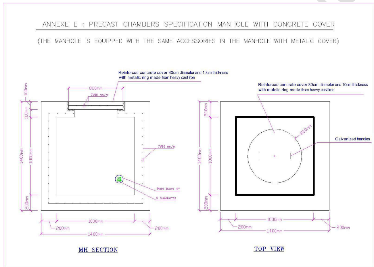
Manhole Specifications & Dimension
