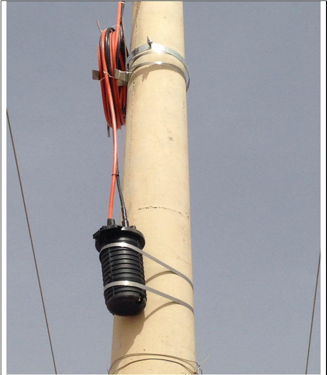
Aerial Cable Storage Configuration for Angled Cables
