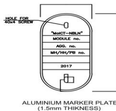
ALUMINIUM MARKER PLATE (1.5mm THICKNESS)
